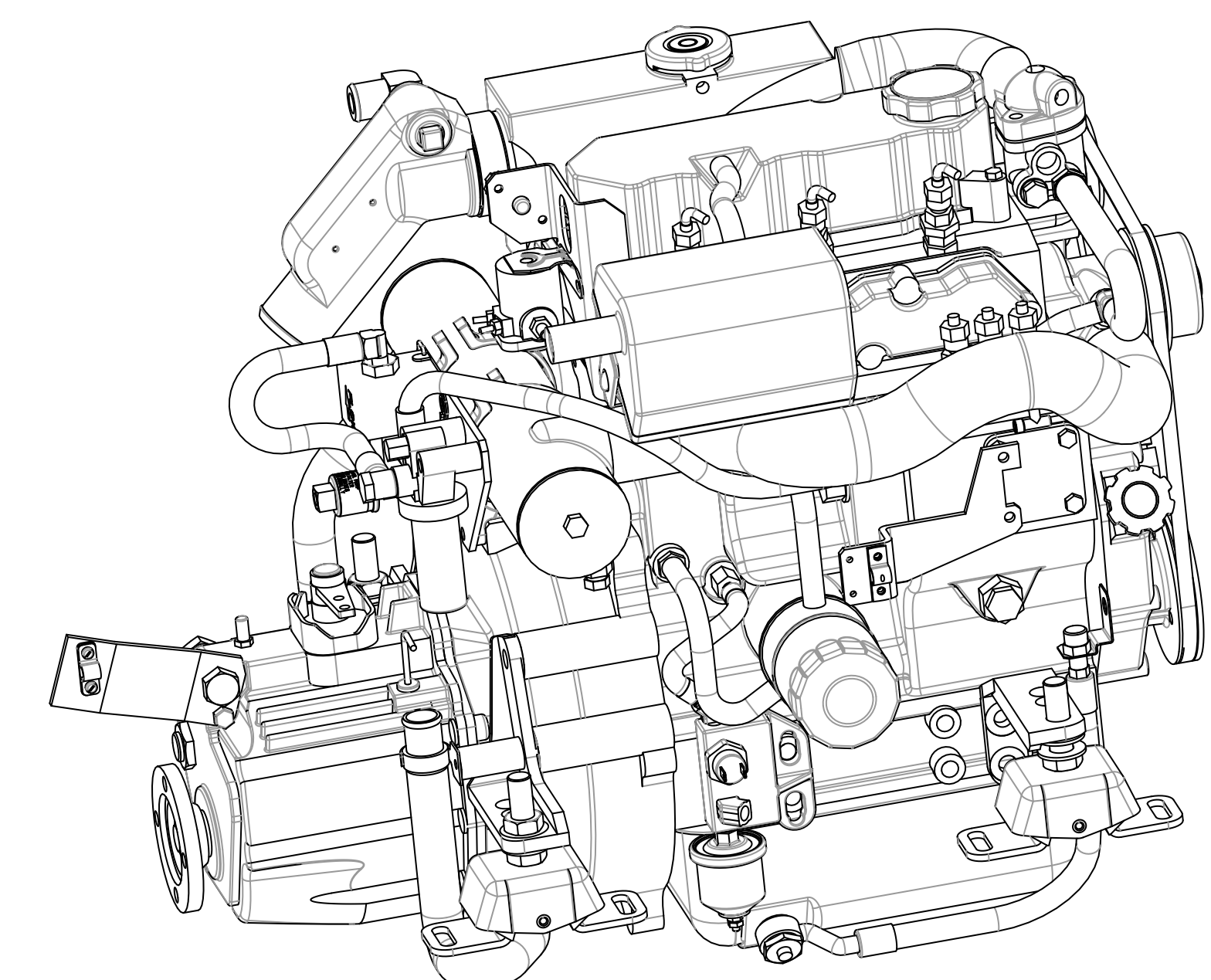
MODEL WITH 50 AMP ALTERNATOR
